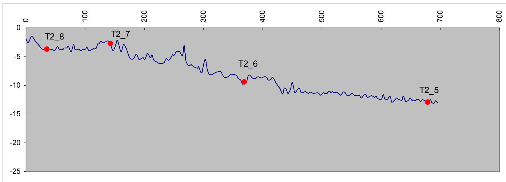
Figure 10. Discovery Bay MNP depth profile for Transect 2 (Figure 8). Video sites extracted from along the transect are labelled on the profile. Depth (y axis) and distance (x axis) are in metres. Note the 0 value on the y axis (depth) represents sea level at the time of the survey.
