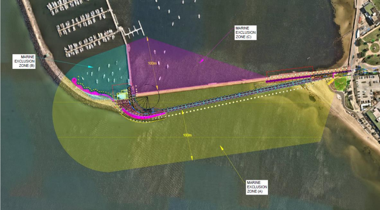
Map 1. St Kilda Pier Redevelopment project works Set Aside areas.
