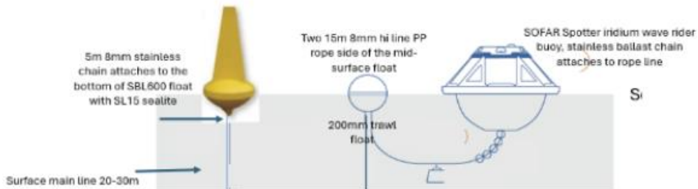
BOUY ARRANGEMENT
