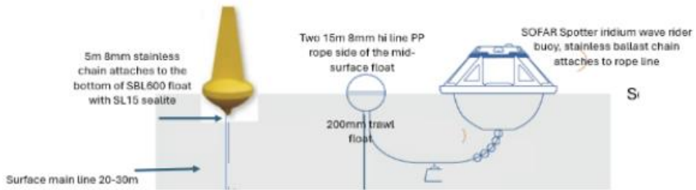
BOUY ARRANGEMENT
